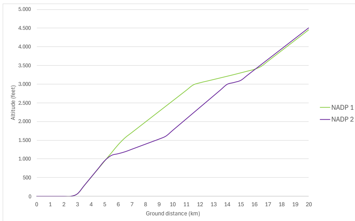
Figure 5.1 Example of the difference between NADP 1 and 2 for a wide body aircraft with thrust reduction at 1,000ft.
