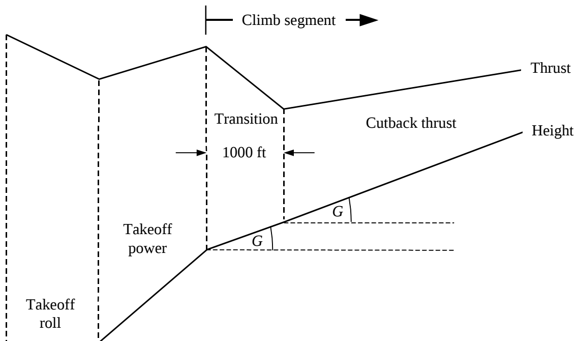
Figure B-2: Constant speed climb segment with cutback (illustration – not to scale)
